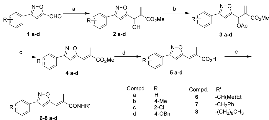
Scheme 1. Reagents and conditions: (a) DABCO (20 mol%), CH 2 =CHCO 2 Me (1.0 equiv), rt, 30 min; (b) AcCl (1.5 equiv), Pyridine (1.3 equiv), DCM, rt, 3 h; (c) NaBH 4 (2.0 equiv), MeOH, rt, 1 h; (d) KOH (2.0 equiv), MeOH: H 2 O (4:1), rt, 2 h; (e) R'NH 2 (1.0 equiv), DIC (1.0 equiv), HOBT (1.0 equiv), DCM, rt, 3–4 h.
