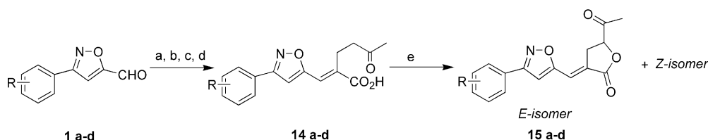
Scheme 4. Reagents and conditions: (a) DABCO (20 mol%), tert -Butyl acrylate (1.0 equiv), rt 30 min; (b) AcCl (1.5 equiv), Pyridine (1.3 equiv), DCM, rt, 2 h; (c) Acetylacetone (2.0 equiv), K 2 CO 3 (1.5 equiv), EtOH, reflux, 2 h; (d) TFA (25%) in DCM, rt, 6 h; (e) HTIB (1.0 equiv), DCM, rt, 16 h.
