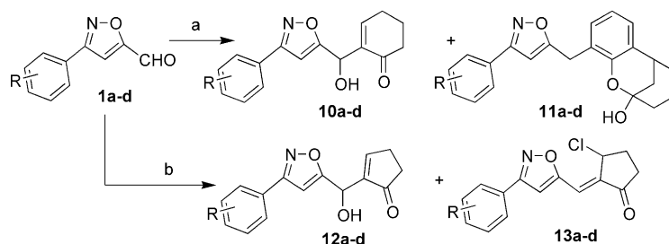
Scheme 3. Reagents and conditions: (a) Cyclohexenone (1.5 equiv), TiCl 4 (1.0 equiv), DCM, rt, 1.5 h; (b) Cyclopentenone (1.5 equiv), TiCl 4 (1.0 equiv), DCM, rt, 1.5 h.
